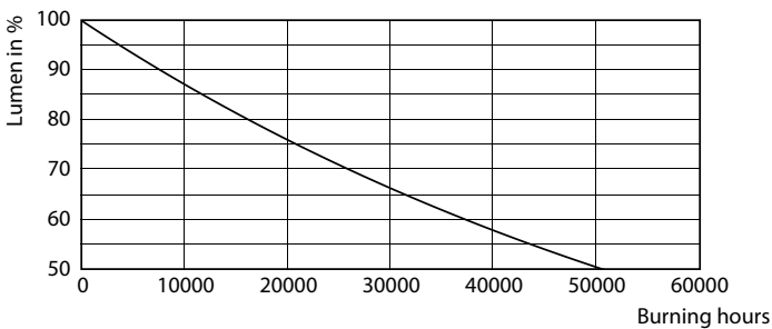
Lumen Maintenance Diagram - LEDBulb 7W E27 6500K W 1PF/40 BR
