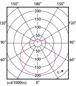
Light Distribution Diagram - LEDBulb 7W E27 6500K W 1PF/40 BR
