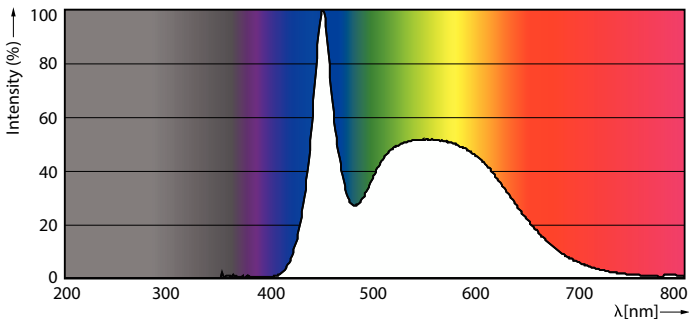
Spectral Power Distribution Colour - LEDBulb 7W E27 6500K W 1PF/40 BR
