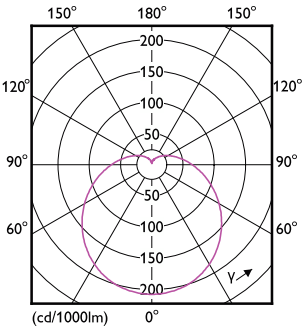
Light Distribution Diagram - LEDBulb 9W E27 3000K W 1PF/40 BR
