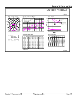
General uniform lighting - LEDBulb 9W E27 3000K W 1PF/40 BR
