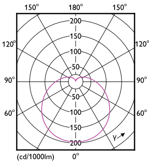
Light Distribution Diagram - LEDBulb 9W E27 6500K W 1PF/40 BR
