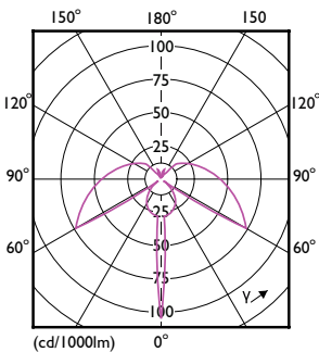
Light Distribution Diagram - LEDBulb 13W E27 3000K W 1PF/40 BR
