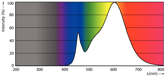
Spectral Power Distribution Colour - LEDBulb 13W E27 3000K W 1PF/40 BR
