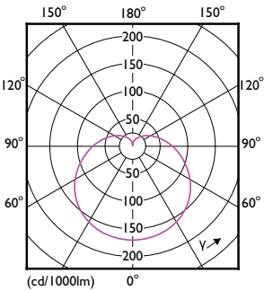
Light Distribution Diagram - LEDBulb 13W E27 6500K W 1PF/40 BR
