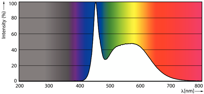
Spectral Power Distribution Colour - LEDBulb 13W E27 6500K W 1PF/40 BR
