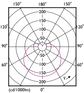
Light Distribution Diagram - LEDBulb 16W E27 3000K W 1PF/40 BR
