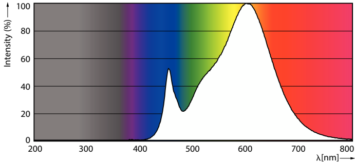
Spectral Power Distribution Colour - LEDBulb 16W E27 3000K W 1PF/40 BR
