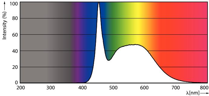
Spectral Power Distribution Colour - LEDBulb 16W E27 6500K W 1PF/40 BR
