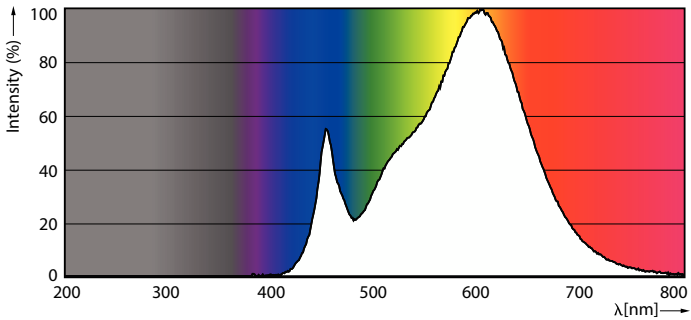
Spectral Power Distribution Colour - LEDBulb 11W E27 3000K W 1PF/40 BR
