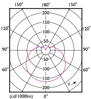
Light Distribution Diagram - LEDBulb 11W E27 3000K W 1PF/40 BR
