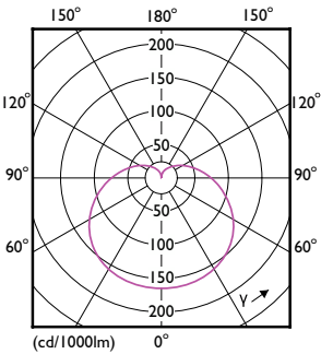
Light Distribution Diagram - LEDBulb 11W E27 6500K W 1PF/40 BR
