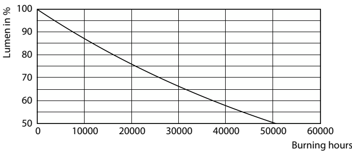
Lumen Maintenance Diagram - LEDBulb 11W E27 6500K W 1PF/40 BR
