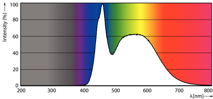
Spectral Power Distribution Colour - LEDBulb 11W E27 6500K W 1PF/40 BR
